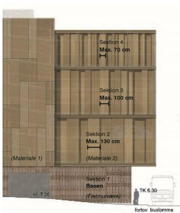
Diagram, Facadebredder
